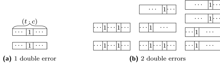
Figure 3: Illustration for the colliding patterns.
