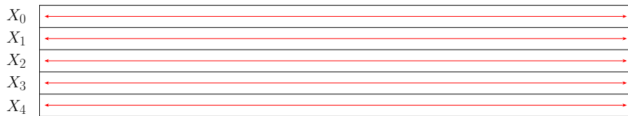
Figure 4: Linear diffusion layer p_L
