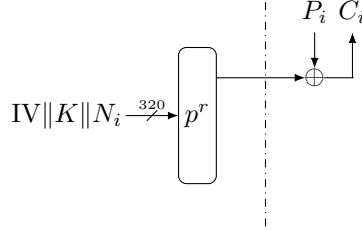
Figure 5: Our attack configuration
