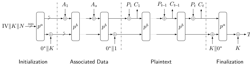
Figure 1: Ascon’s mode of operation (encryption phase)
