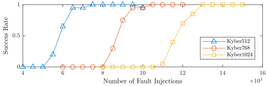
Figure 10: Attack success rate for all 3 Kyber parametrizations as function of faulted decapsulations
