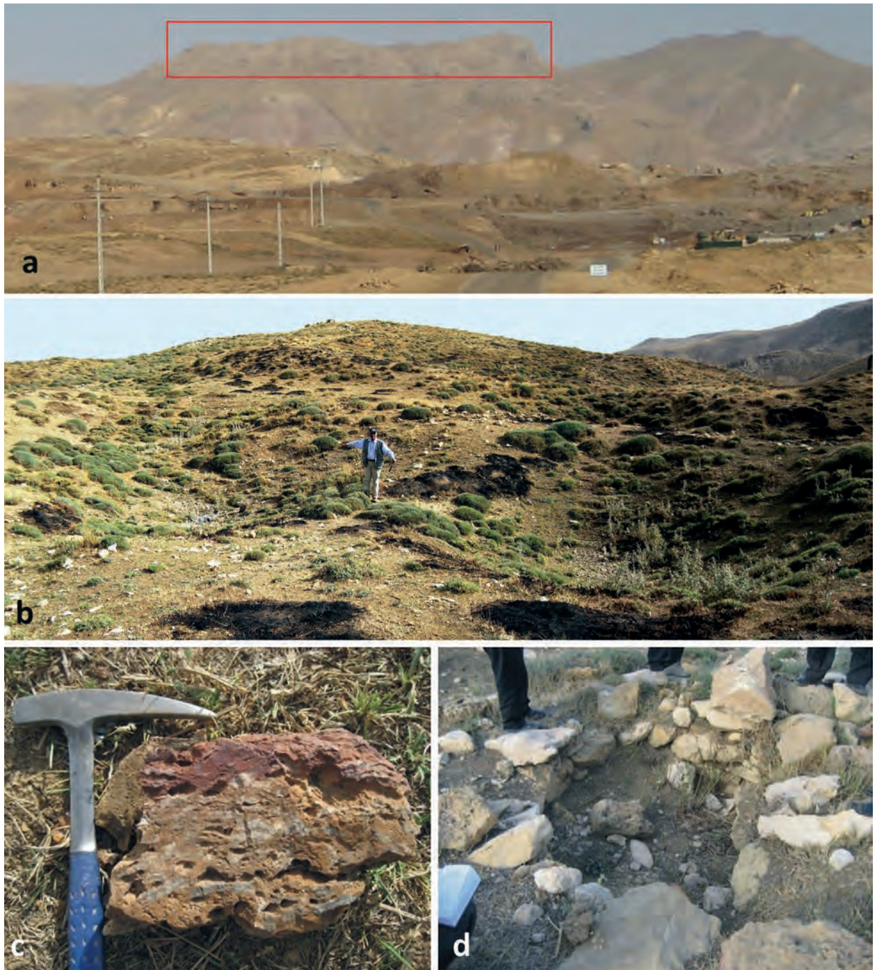
Figure 6: a) an overview of the Shakh-Shakh ancient mining area situated in the high mountains, b) ancient diggings as shallow conical depressions, c) cinnabar mineralization with silica as found in an ancient diggings, d) a possible entrance of an ancient diggings.
